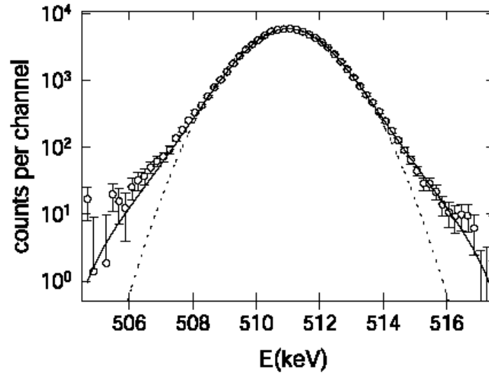
Fig. 7. (open circles) Doppler-broadened gamma-ray spectrum from positron annihilation on helium atoms and comparison with (—) theoretical predictions using a variational wavefunction, and (---) a Gaussian fit. From Ref. [33].
