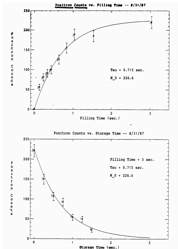
Fig. 4. Data from a trapping experiment in August 1987. Above: number of positrons confined as a function of fill time, maximum number \sim 1 \times 10^4 . Below: confinement as a function of time after the fill was turned off, indicating a 0.7 s confinement time. The confinement was limited by annihilation on a very low density of large, molecular impurities at pressures < 10^{-9} torr.
