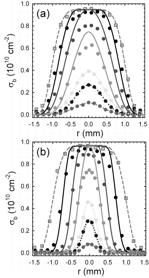
Figure 2.7: Profiles \sigma_b(r) of extracted beams: (a) T \approx 1.0 \text{ eV} , \xi \approx 0.1, 0.3, 0.5, 1.0, 1.9, 2.8 ; and (b) T \approx 0.2 \text{ eV} , \xi \approx 0.1, 0.3, 0.5, 2.2, 5.2, 11 . In both (a) and (b), the three smallest beams are fit ( \cdots ) to Eq. 2.14, and the three largest beams are fit ( \text{---} ) to numerical solutions to Eqs. 2.4 and 2.5. The initial plasma profile \sigma_z(r) is shown ( \square ), as is the fit ( \text{- - -} ) used in the numerical solutions.
