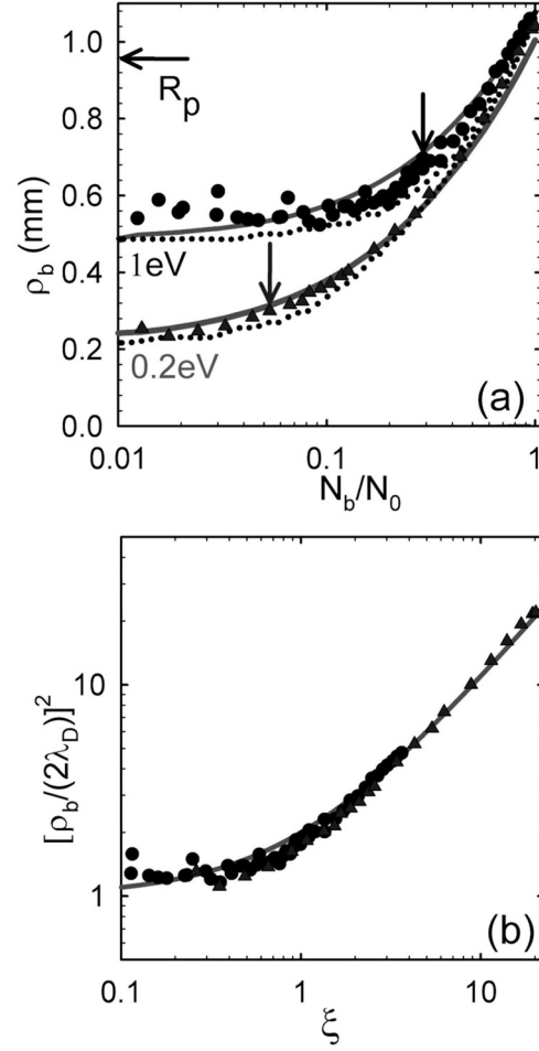
Figure 2.8: (a) Beam width parameter \rho_b plotted vs. N_b/N_0 for T \approx 1.0 eV ( \bullet ), and 0.2 eV ( \blacktriangle ). Predictions (—) from Eq. 2.15 with no fitted parameters, and ( \cdots ) numerical solutions to Eqs. 2.4 and 2.5. Arrows correspond to beams with \xi = 1 . (b) Data from (a) plotted as (\rho_b/2\lambda_D)^2 vs. \xi , showing all data lies on a single curve (—) given by Eq. 2.15.
