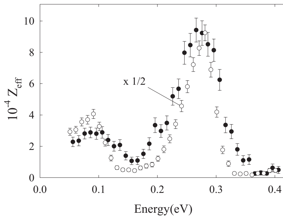
Figure 5.2: Z_{eff} spectra for ( \circ ) hexane, scaled by 1/2, and ( \bullet ) cyclohexane.
