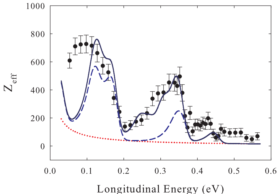
Figure 4.6: Z_{\text{eff}} for methanol, with adapted Gribakin-Lee model predictions, assuming 2 meV positron binding energy. The dotted curve represents the non-resonant (direct) contribution; the dashed line represents the total contribution including only fundamental-mode VFRs; and the solid curve represents the total contribution including both fundamental and multi-mode VFRs. Theoretical results were provided by G. Gribakin (private communication). See text for details.
