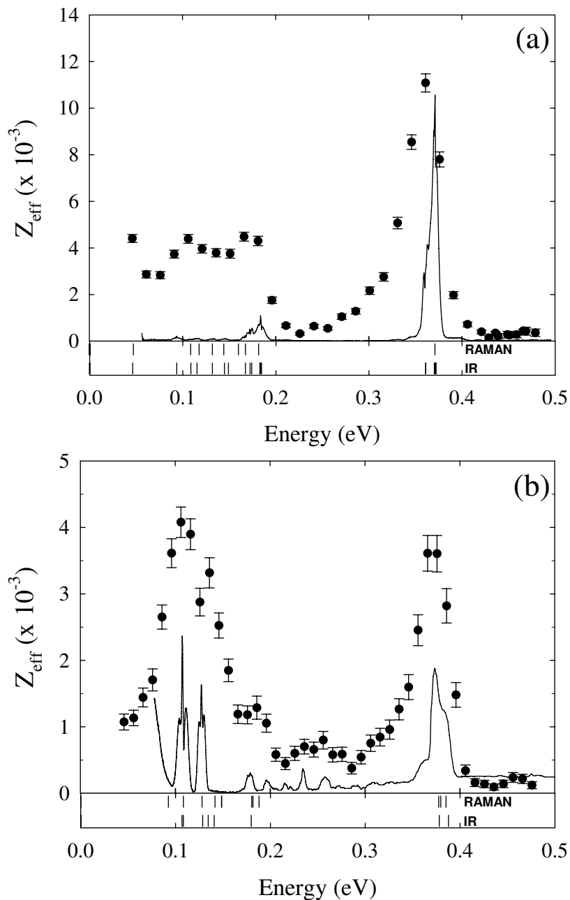
Figure 4.11: Energy-resolved Z_{\text{eff}} ( \bullet ) for (a) propane and (b) cyclopropane. The solid curve ( - ) represents normalized IR absorption and the vertical bars below each plot show the active vibrational mode energies, both from Ref. [66].
