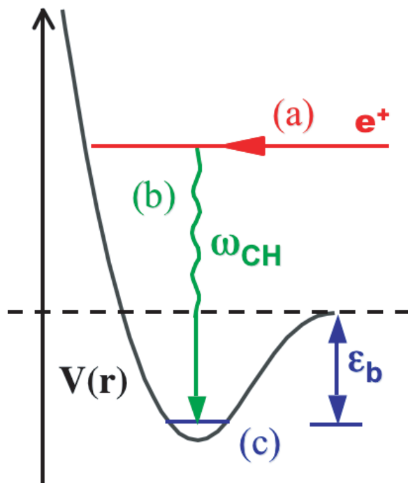
Figure 2.3: A cartoon of the VFR model consisting of three steps: (a) the positron approaches the molecule along coordinate r with energy \omega_\nu - \epsilon_b ; (b) the positron excites a molecular vibration of energy \omega_\nu ; and simultaneously, (c) the positron drops into a positron-molecule bound state of depth \epsilon_b where it may annihilate with molecular electrons. Note that this is merely a qualitative representation of the interaction which ignores all other degrees of freedom outside of the positron approach coordinate r .
