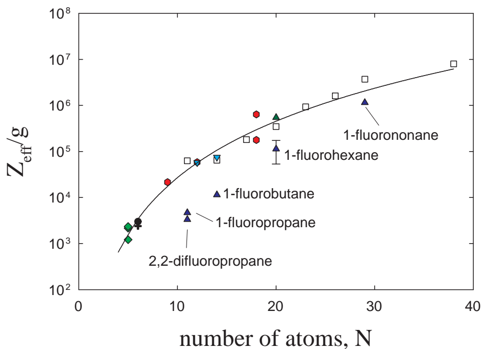
Figure 5.10: Normalized Z_{eff} at the C-H stretch peak vs number of atoms for a variety of species (similar to Fig. 5.5), including (blue \triangle ) suppressed- Z_{eff} molecules. The error bars on 1-fluorohexane indicate the unusually large uncertainty in this datum. The solid line shows the previously described Z_{eff}/g = 2.3 N^{4.1} fit for non-suppressed molecules.
