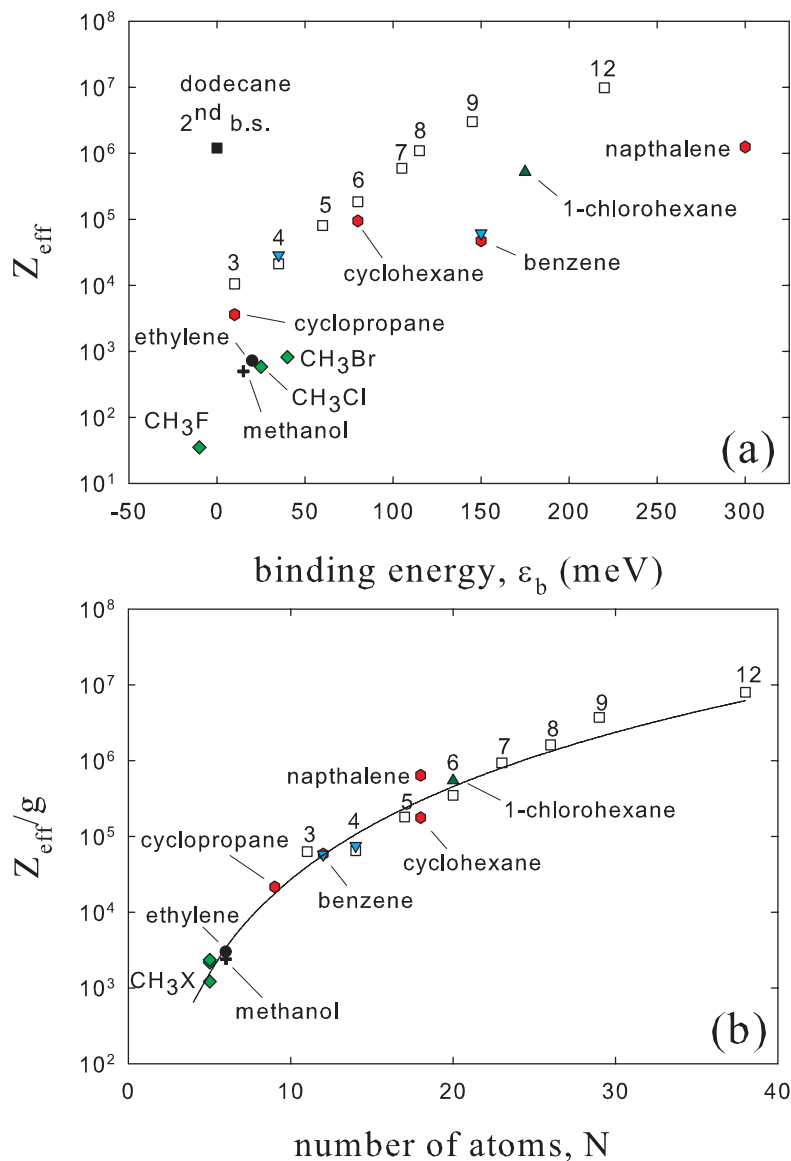
Figure 5.5: (a) Z_{\text{eff}} at the C-H stretch peak vs binding energy, \epsilon_b , for alkanes, \text{C}_n\text{H}_{2n+2} ( \square ); rings (red hexagons); halomethanes (green \diamond ); ethylene ( \bullet ); methanol (+), 1-chlorohexane (dark green \triangle ); and deuterated species (cyan \nabla ). (b) Z_{\text{eff}} at the C-H stretch peak normalized by the factor g = \sqrt{\epsilon_b/\epsilon} vs the number of atoms, N , in the molecule. For alkanes, the number of carbon atoms, n is indicated. In (b), the solid line shows the fit, Z_{\text{eff}}/g = 2.3 N^{4.1} , described in the text. This plot demonstrates that Z_{\text{eff}} is insensitive to positron binding beyond the weak dependence, g , which is predicted by theory.
