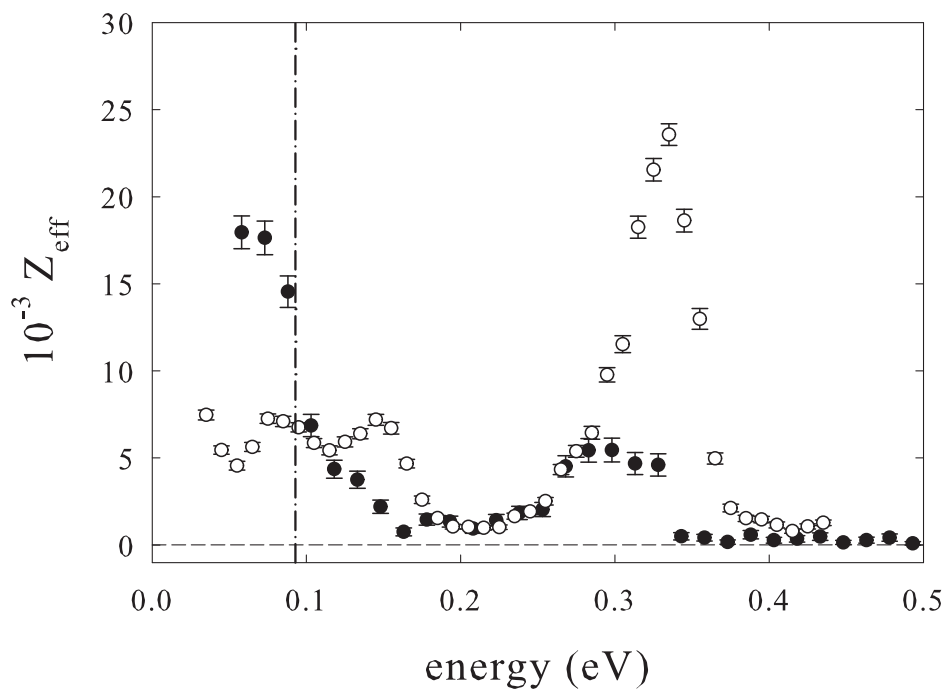
Figure 5.9: Z_{\text{eff}} spectra for ( \circ ) butane and ( \bullet ) 1-fluorobutane. The vertical dot-dash line ( -\cdot- ) indicates the empirical position of a inelastic threshold (explained in a later section).
