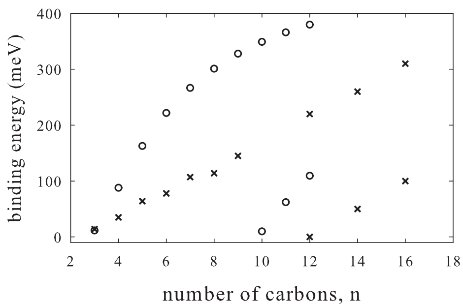
Figure 5.15: ZRP model for binding energy in alkanes ( C_nH_{2n} ) as a function of the number of carbons, n (reproduced from Ref. [65]). This plot shows the theoretical binding energies ( \circ ) for a chain of ZRP monomers as well as experimental binding energies ( \times ) for the first and second bound states in alkanes [43, 45, 70].
