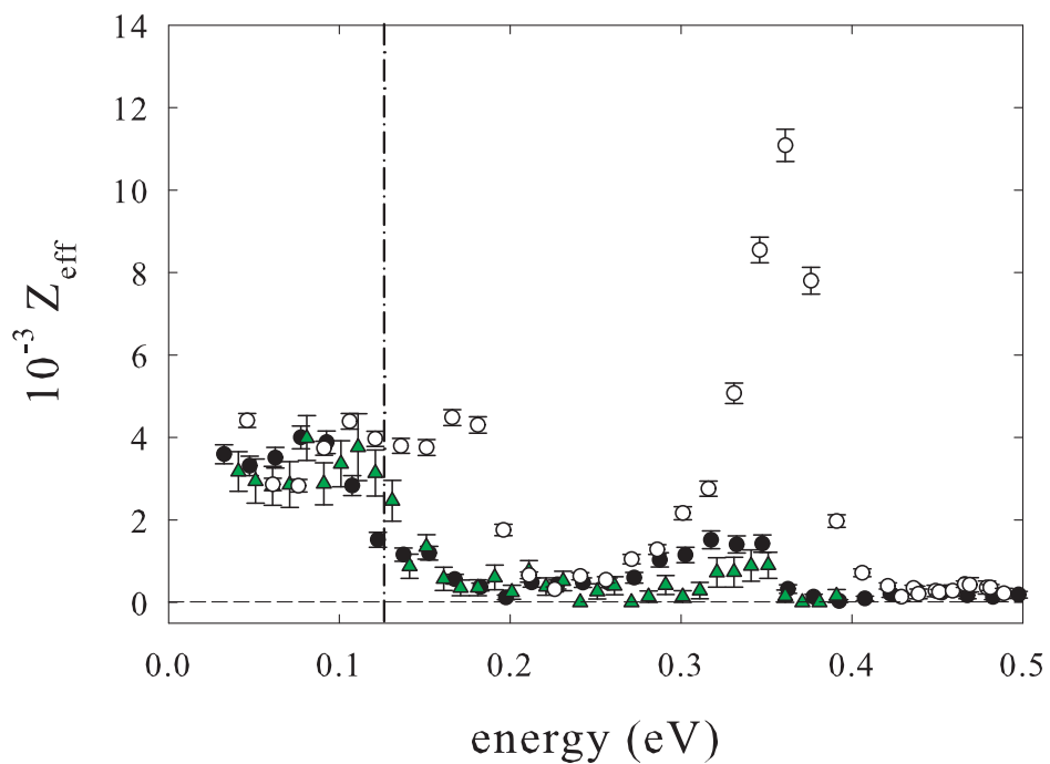
Figure 5.8: Z_{\text{eff}} spectra for (○) propane and (●) 1-fluoropropane (present work), and (green \triangle ) 2,2-difluoropropane from Ref. [24]. The vertical dot-dash line (---) indicates the empirical position of an inelastic threshold – roughly where the Z_{\text{eff}} magnitude is reduced to half of its low energy value, averaged between the two fluorinated species. This is explained in a later section.
