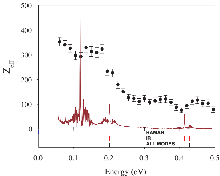
Figure 4.8: Energy-resolved Z_{eff} and infrared absorption spectra for ammonia reproduced from Ref. [62]. The bars below indicate the positions of vibrational modes (from Ref. [66]).
