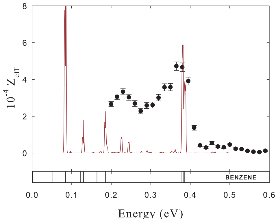
Figure 5.11: Energy-resolved Z_{eff} (●) and infrared absorption (—) for benzene. The Z_{eff} has been shifted upward by the binding energy \epsilon_b = 150 for direct comparison. The IR absorption, from Ref. [66], is arbitrarily normalized. The lower panel indicates the positions of the vibrational modes in benzene from Ref. [66].
