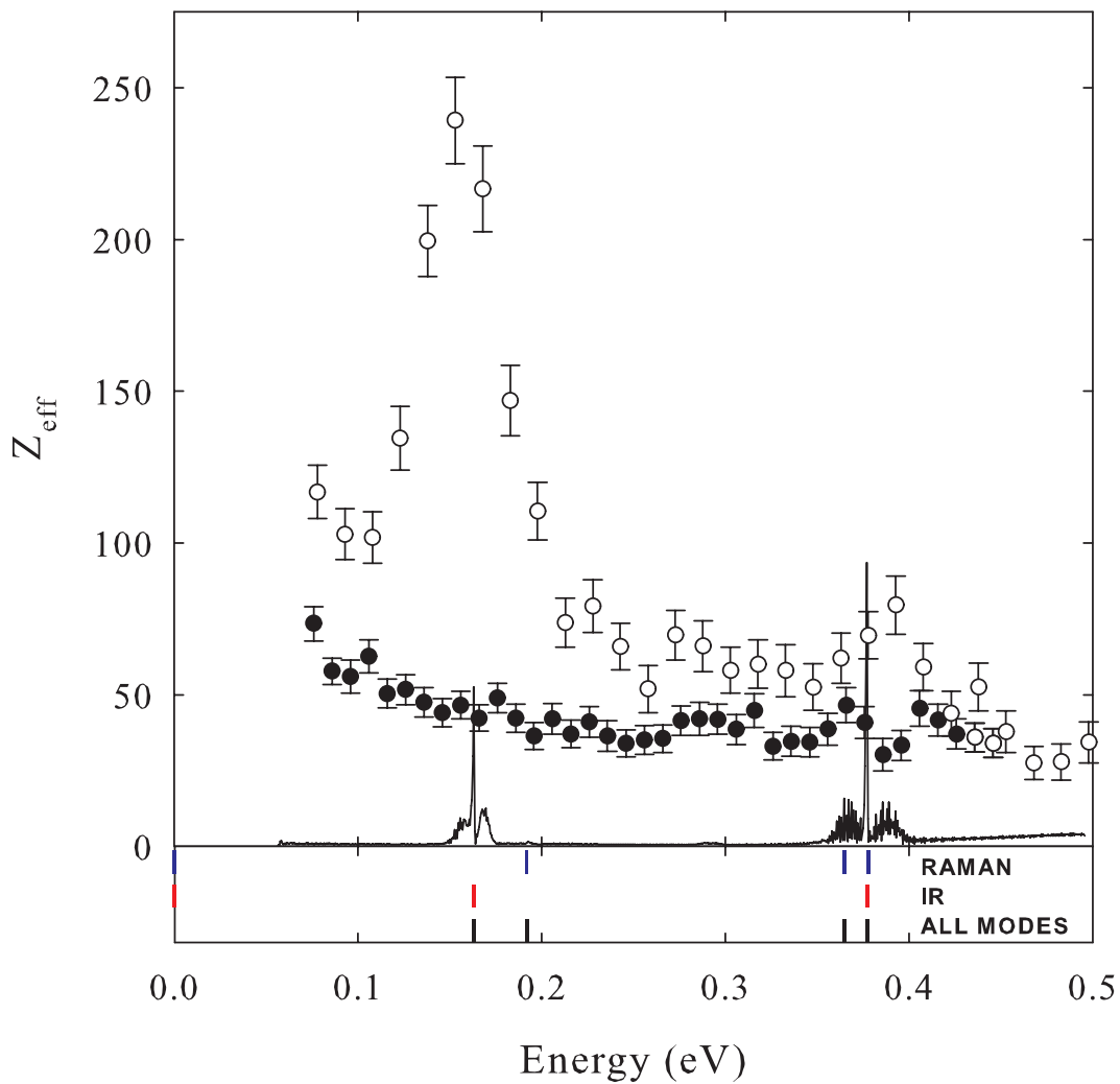
Figure 4.12: Energy-resolved Z_{\text{eff}} for (●) CH 4 and (○) CH 3 F from Ref. [43]. The solid curve (—) represents normalized IR absorption for CH 4 and the vertical bars below this plot show the active vibrational mode energies for CH 4 , both from Ref. [66]. Note the lack of VFR in CH 4 as compared to CH 3 F.
