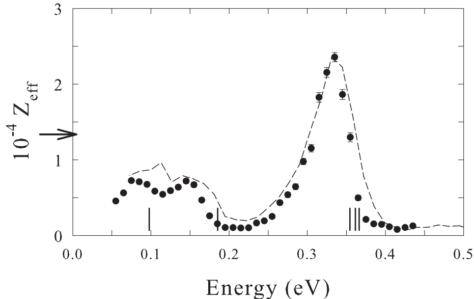
Figure 2.2: Energy-resolved Z_{eff} for ( \bullet ) butane and (---) scaled d-butane from [24]. The d-butane energy is scaled empirically by a factor nearly equal to the ratio of C-H and C-D stretch mode energies (after correcting for binding). The magnitude of this curve is normalized arbitrarily. The arrow on the ordinate indicates the thermal Z_{eff} for butane. The vertical bars at the bottom indicate the energies of fundamental vibrational modes. See Ref. [24] for details.
