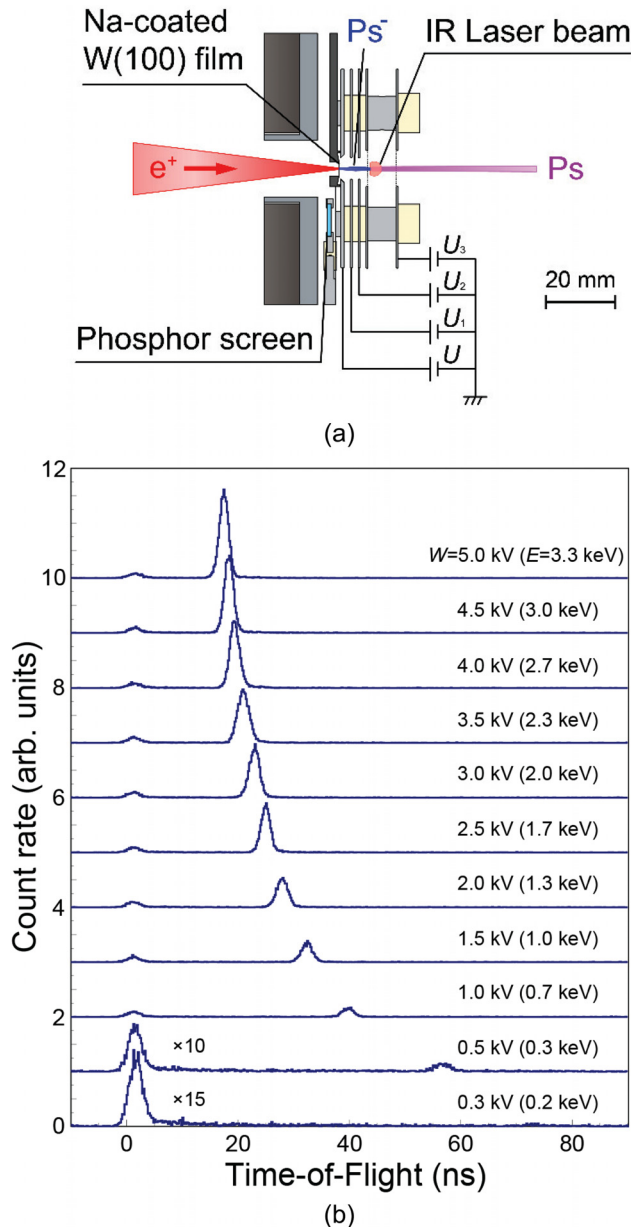
FIG. 14. Formation of a variable-energy Ps beam using Ps - ions. 98 (above) Schematic diagram of the apparatus. A pulsed positron beam from a BGT is focused on a Na-coated W film, which emits Ps - ions. The ions are accelerated through an imposed potential drop V and then laser stripped to form the Ps beam. (below) Time-of-flight energy spectra of the resulting beam upon varying V from 0.3 to 5.0 kV. Reproduced with permission from Rev. Sci. Instrum. 90 , 023305 (2019). Copyright 2019 AIP Publishing. 98
