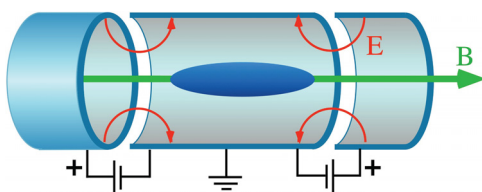
FIG. 1. Schematic diagram of a Penning-Malmberg trap for the confinement of plasmas consisting of particles of a single sign of charge, here biased for positive charges. Typical electrode radii and lengths are several centimeters. The “parallel” direction z is defined to be aligned with the trap and magnetic axes, and “perpendicular” refers to the orthogonal directions.
