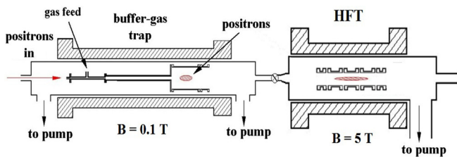
FIG. 2. Schematic diagram of a three-stage buffer-gas positron trap and an adjacent high-magnetic-field UHV trap (HFT). In the BGT, each of the latter two stages are at successively lower buffer-gas pressures and lower electrical potentials.
