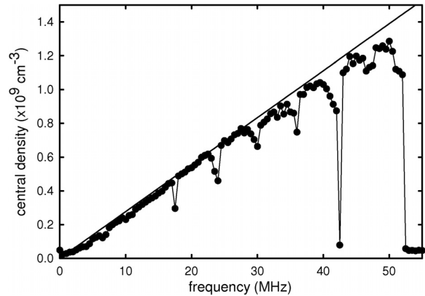
FIG. 9. Change in the density of a positron plasma as a function of the applied RW frequency when a constant frequency is applied. 15 The solid line corresponds to f_E = f_{RW} , characteristic of the strong drive regime. For this experiment, B = 0.04 T, and the maximum density achieved is 17% of the Brillouin density limit. The sharp drops in the density at specific frequencies are due to the static asymmetries that couple to low-order plasma modes and act as a drag on the plasma. Reprinted with permission from Danielson and Surko, Phys. Rev. Lett. 94 , 035001 (2005). Copyright 2005 American Physical Society. 74
