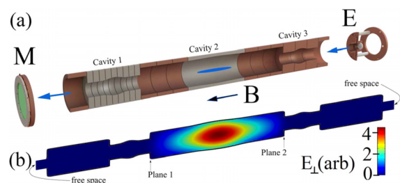
FIG. 4. (a) Electrodes of a PM trap designed to exploit the resonant-cavity cyclotron cooling in resonant cavity 2. Cavities 1 and 3 act as waveguides beyond cutoff. (b) The simulated electric field intensity for the TE_{111} mode in cavity 2. Reproduced with permission from Phys. Plasmas 25, 011602 (2018). Copyright 2018 AIP Publishing. 56
