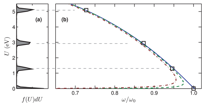
FIG. 11. Autoresonant release of a cloud of antiprotons from a potential well. The frequency is swept downward from the linear value for this well with bounce frequency \omega_0/2\pi = 410 kHz. The open squares (right) denote the mean beam energy U of each distribution f(U) (left), plotted against the final drive frequency (dashed lines). Reprinted with permission from Andresen et al. , Phys. Rev. Lett. 106 , 025002 (2011). Copyright 2011 American Physical Society. 79
