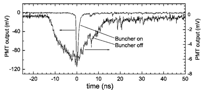
FIG. 12. Positron pulses with and without a harmonic buncher, showing the time compression of a factor of approximately 10 to <2 ns. Reproduced with permission from Rev. Sci. Instrum. 77, 073106 (2006). Copyright 2006 AIP Publishing. 89
