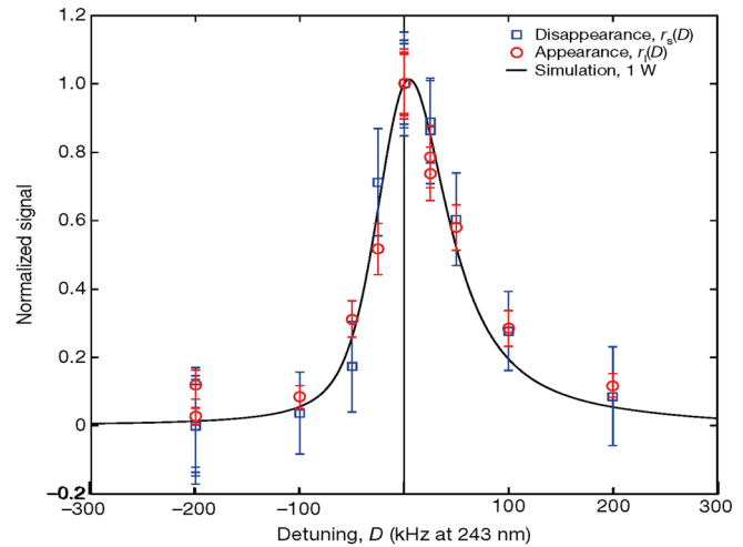
FIG. 15. A measurement of the antihydrogen two-photon 1S-2S transition is shown here corresponding to a relative precision of 2 \times 10^{-12} . 9 The points show the number atoms that are detected (appearance) when “kicked” out of the system after illumination by light at various detuning frequencies, and the number of atoms that are missing (disappearance) after illumination as inferred by subtracting the number remaining after illumination from the number before illumination (done with multiple, repeated ensembles). The line is the result of a simulation with 1 W of laser power. From Ref. 9.
