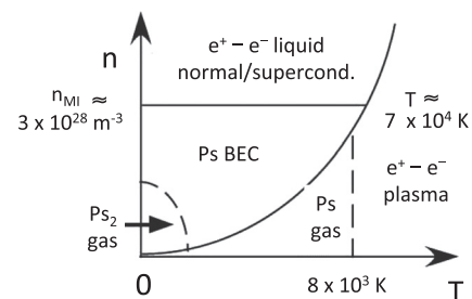
FIG. 16. Schematic (only) phase diagram of the electron-positron system as a function of density n and temperature T . The density n_{\text{MI}} of the metal-insulator transition is indicated. While this quantum phase is beyond the current technology, \text{Ps}_2 has been created and studied, and near-term studies of a Ps BEC and a classical pair plasma are possible. Adapted from Ref. 122.
