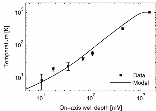
FIG. 6. (a) Six steps of evaporative cooling of antiprotons, resulting in a temperature decrease from 1000 K to 9 K (■). The temperature vs the on-axis well depth is compared with a model calculation (solid line). The initial number of antiprotons was approximately 45 000 at an on-axis well depth of 1.5 eV. Approximately 6% of the particles remain at the final temperature of 9 K. Reprinted with permission from Andresen et al. Phys. Rev. Lett. 105 , 013003 (2010). Copyright 2010 American Physical Society. 53
