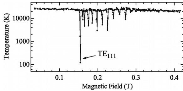
FIG. 5. Measured temperatures of electron plasmas initially at 26 000 K and cooled for 8 s at the indicated magnetic field values using the apparatus in Fig. 4. The dips occur upon the excitation of TE_{11X} modes. Reproduced with permission from Phys. Plasmas 25 , 011602 (2018). Copyright 2018 AIP Publishing. 56
