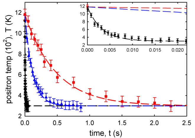
FIG. 3. Positron cooling on molecular vibrations and rotations for (black filled circle) CF_4 (blue filled triangle), CO, and (brown filled square) N_2 gases at 300 K (horizontal line). 52 The data are normalized to 1 \mu\text{Torr} and shifted to coincide at t = 0 s; the dashed lines show an exponential fit for each case. The inset shows CF_4 in more detail. The corresponding cooling times to 1/e are 4.8, 130, and 1500 \text{ ms}/\mu\text{Torr} for CF_4 , CO, and N_2 , respectively. Reproduced with permission from Natisin et al. , J. Phys. B 47, 225209 (2014). Copyright 2014 IOP Publishing. 52
