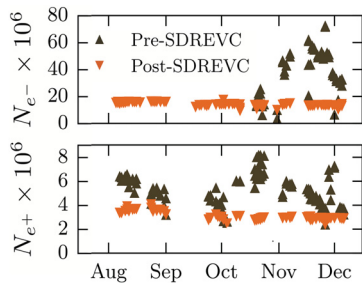
FIG. 10. Stability of the electron and positron plasmas (the former for the sympathetic cooling of the antiprotons) used to create antihydrogen atoms before and after plasma tailoring by radial compression and evaporative cooling (SDREVC). Reprinted with permission from Ahmadi et al. , Phys. Rev. Lett. 120 , 025001 (2018). Copyright 2018 American Physical Society. 62
