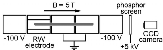
FIG. 7. Apparatus for the RW compression of single component, negatively charged plasmas. The areal density profile is measured by accelerating the particles onto a phosphor screen and measuring the resulting light, as discussed in Sec. III. Reprinted with permission from Danielson and Surko, Phys. Rev. Lett. 94 , 035001 (2005). Copyright 2005 American Physical Society. 74
