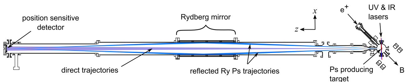
FIG. 13. Transmission and focusing of a high-Rydberg-state Ps beam. 105 Stark Ps states are formed using a UV and an IR laser. They are reflected from, in particular, a prepared "Rydberg mirror" consisting of closely spaced rods approximately parallel to the beamline with alternating DC potentials that create a localized electric field near the surface. The mirror has a slight curvature such that low-field seeking Ps states are focused on a detector 6 m from the Ps source. Reprinted with permission from Jones et al. , Phys. Rev. Lett. 119 , 053201 (2017). Copyright 2017 American Physical Society. 105
