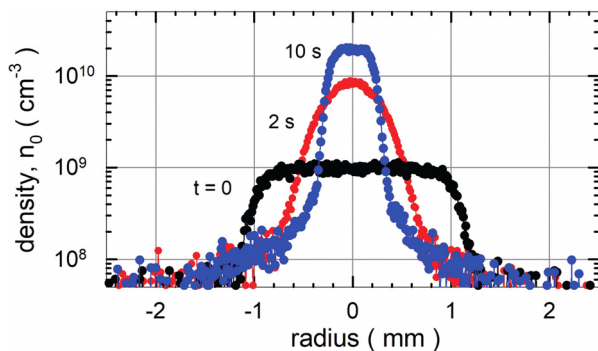
FIG. 8. Rotating wall compression of an electron plasma starting at time t = 0 . 74 Note the log density scale. The constant density profiles at t = 0 and 10 s are characteristic of a rigid-rotor rotational motion [i.e., as described by Eq. (2)]. Reprinted with permission from Danielson and Surko, Phys. Rev. Lett. 94 , 035001 (2005). Copyright 2005 American Physical Society. 74
