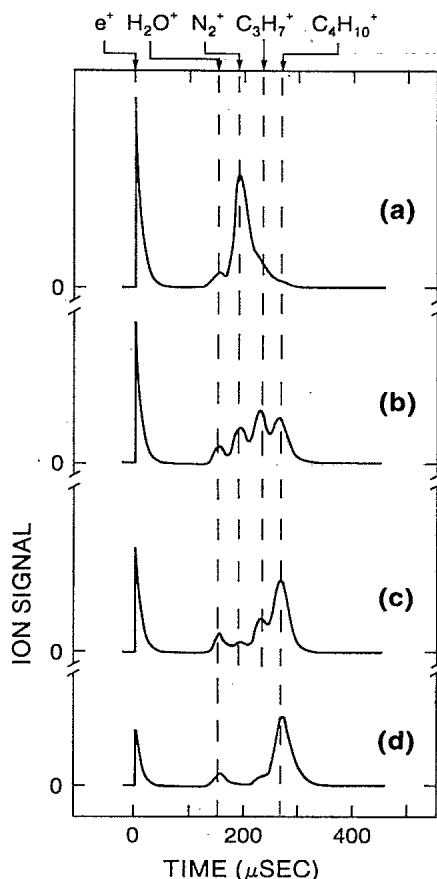
FIG. 1. Time-of-flight spectra of the ions when butane is present in the positron trap. The filling time was 0.5 s, the N_2 pressure was 0.5 \times 10^{-7} torr, and the butane pressure was 2.5 \times 10^{-7} torr. The traces correspond to storage times of (a) 0 s, (b) 0.5 s, (c) 1 s, and (d) 2 s. The identification of the peaks and their expected positions are indicated.
