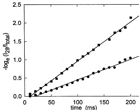
FIG. 2. The decay of the N_2^+ ion signal versus time in an ion-trap mass spectrometer in the presence of (■) butane at a pressure of 3.5 \times 10^{-7} torr and (●) heptane at a pressure of 9.7 \times 10^{-8} torr.
