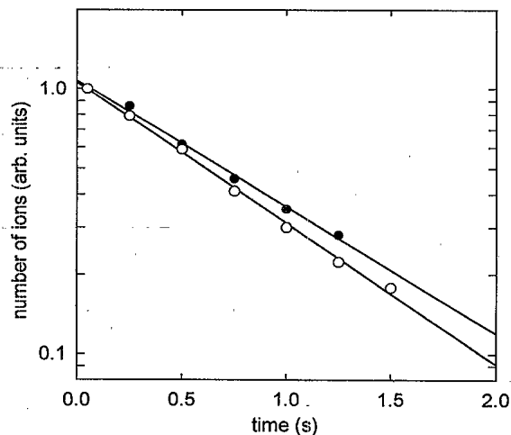
FIG. 5. Number of ions remaining in the Penning trap as a function of storage time for a magnetic field of 1075 G: (○) nitrogen and (●) butane. These data were taken under conditions where each ion species was dominant. Fits to exponentials give confinement times of \tau = 0.82 and 0.91 s for nitrogen and butane, respectively.
