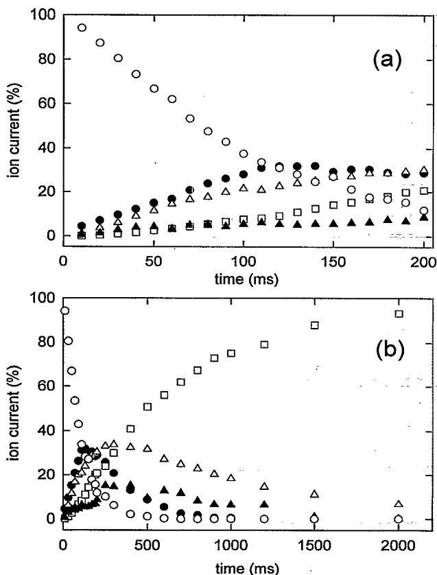
FIG. 4. Ion currents as a function of time, measured in an ion-trap mass spectrometer, for the reaction of N_2^+ ions with butane: (a) 0–0.2 s, and (b) 0–2 s; for (○) N_2 , (●) C_2 , (△) C_3 , (□) C_4 , and (▲) H_2O .
