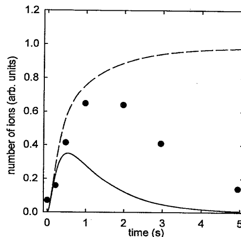
FIG. 6. Number of butane ions remaining in the positron trap as a function of storage time. The solid points are from Ref. [1]. All data are normalized to the number of nitrogen ions at time t=0 . The expected signal from reactions (1)–(5) is shown by the solid line. The dashed line is that expected from reactions (1)–(5) if the ion confinement time were long compared to the time scale of the experiment.
