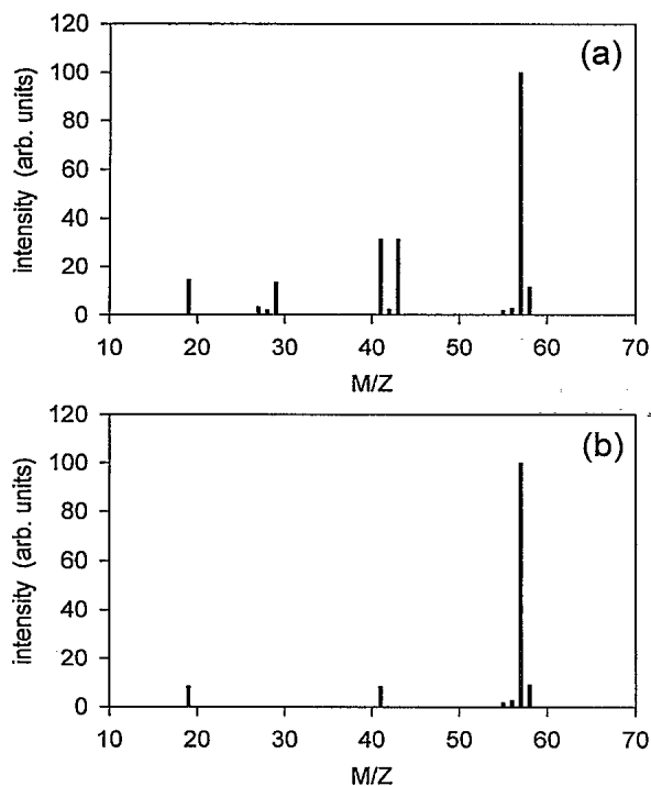
FIG. 3. Mass spectra for the reaction of N_2^+ with butane, studied in an ion-trap mass spectrometer: (a) 0.5-s reaction time and (b) 1.0-s reaction time.
